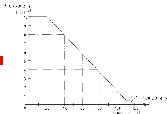
Temperature-Pressure Diagram
